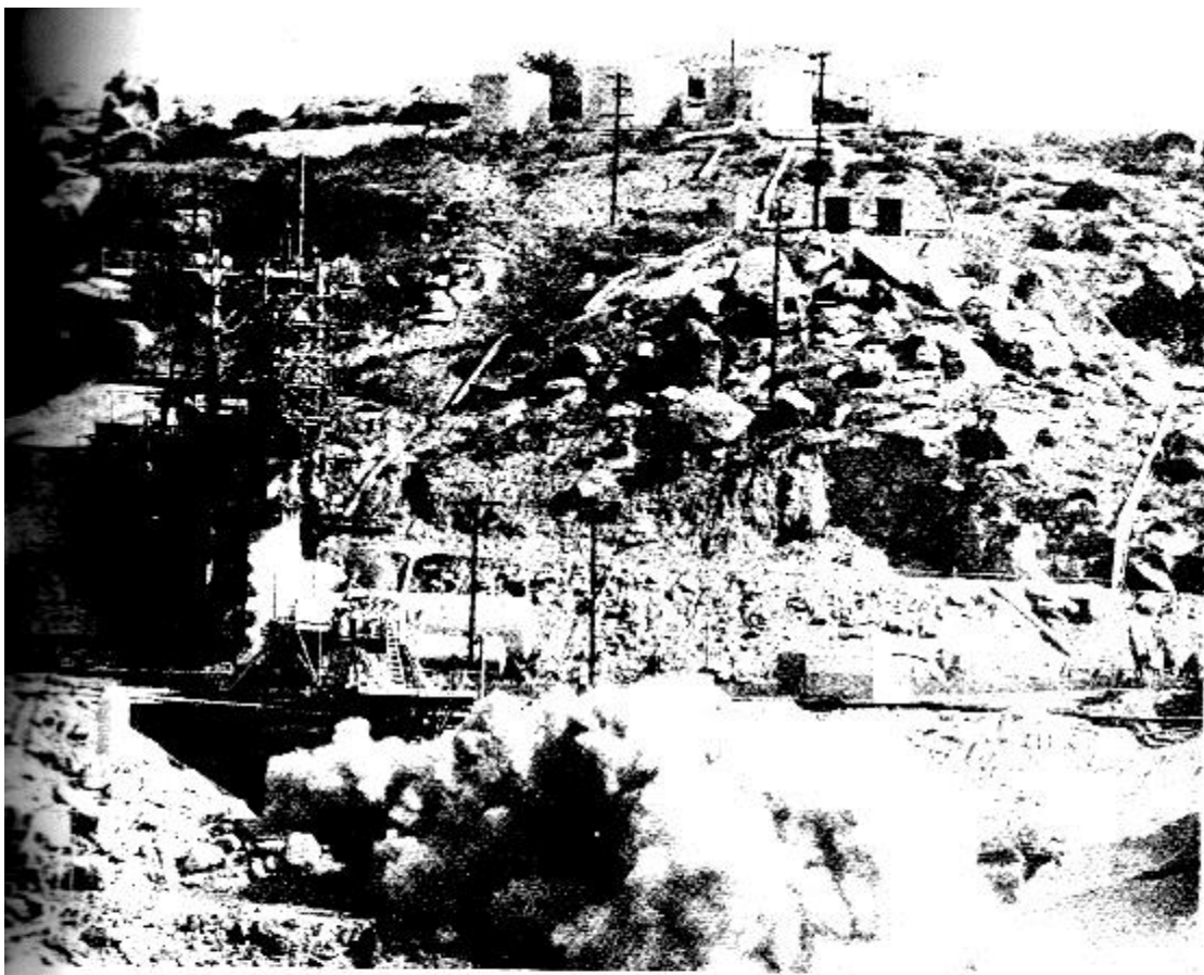
A test of hypergolic propellants: nitrogen tetroxide and hydrazine (UDMH) at the Field Lab. Such tests were dangerous in the extreme due to the toxicity of the propellants in their burned or unburned state. The residents of the nearby San Fernando Valley were not told of the nature or danger of this type of testing -- another example of the cavalier attitude of large corporations.
